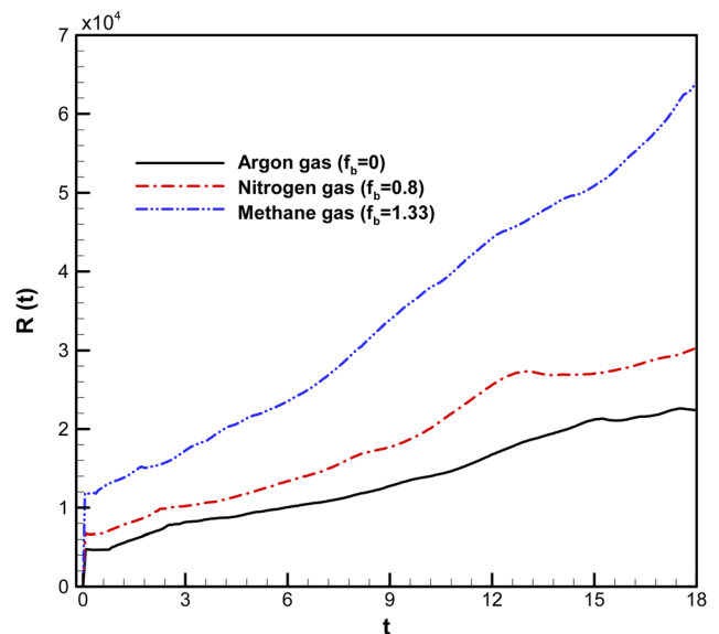
FIG. 16. Effects of diatomic and polyatomic gases on the shock-accelerated cylindrical He bubble: spatially integrated fields of degree of thermal non-equilibrium.
