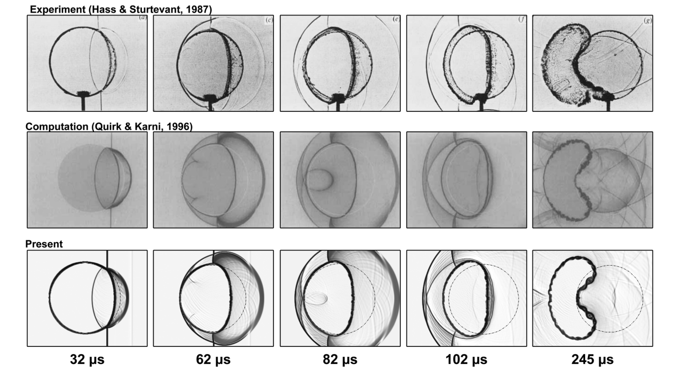
FIG. 6. Validation of the numerical solver: comparison of numerical schlieren images between the experimental results [reproduced with permission from J. F. Haas and B. Sturtevant, J. Fluid Mech. 181, 41–76 (1987). Copyright 1987 Cambridge University Press], 13 the computational results [reproduced with permission from J. J. Quirk and S. Karni, J. Fluid Mech. 318, 129–163 (1996). Copyright 1996 Cambridge University Press], 20 and the present numerical results for a shock-accelerated R 22 cylindrical bubble surrounded by air at different time instants.
