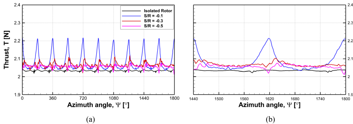
FIG. 17. Comparison of time-history of thrust forces between isolated rotor and rotor-conical airframe configurations with different separation distances: (a) 5 rev. and (b) 1 rev.
