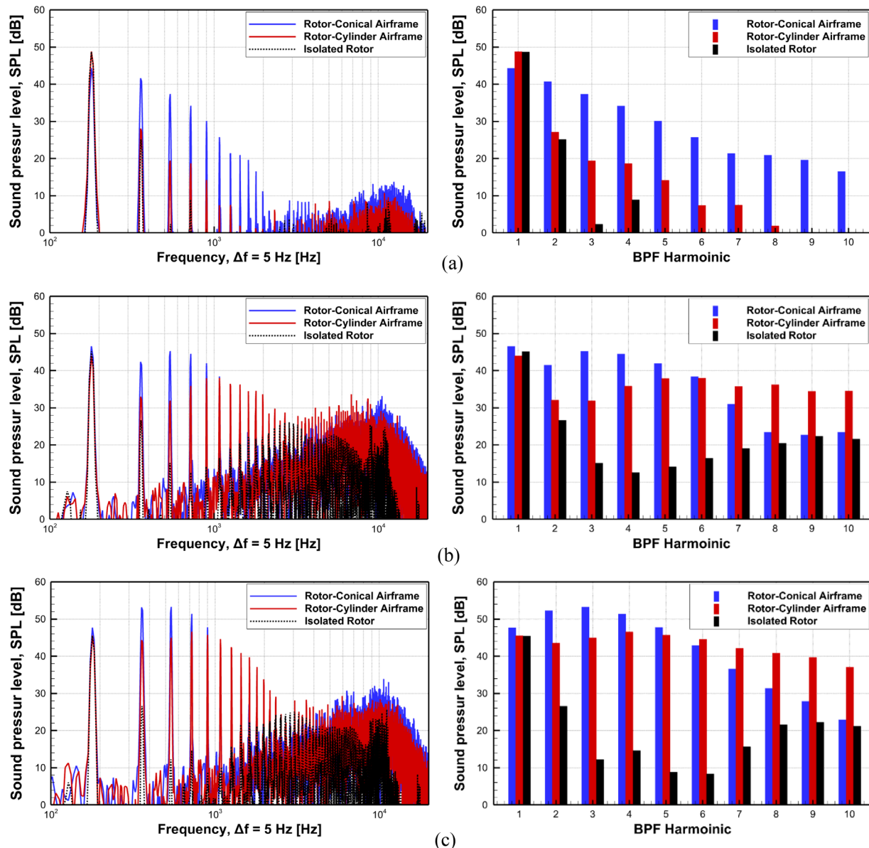
FIG. 14. Acoustic narrowband spectra (left) and BPF harmonics (right) comparisons between rotor–airframe and isolated rotor configurations: (a) M1, (b) M3, and (c) M5 locations.
