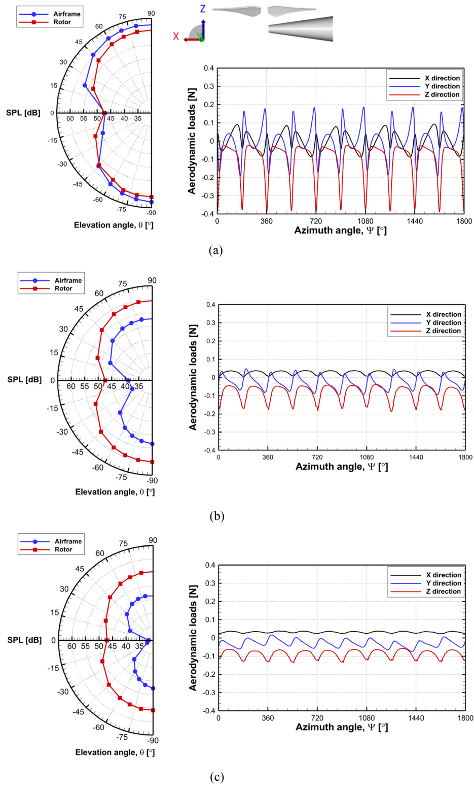
FIG. 22. Comparison of noise contributions (left) and time-history of force acting on the airframe (right) depending on the separations distance: (a) S/R = -0.1 , (b) S/R = -0.3 , and (c) S/R = -0.5 .
