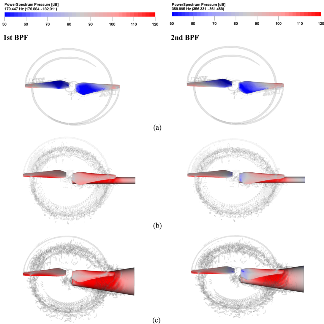
FIG. 15. Comparison of dB surface map at first BPF (left) and second BPF (right): (a) isolated rotor, (b) rotor-cylinder airframe, and (c) rotor-conical airframe.
