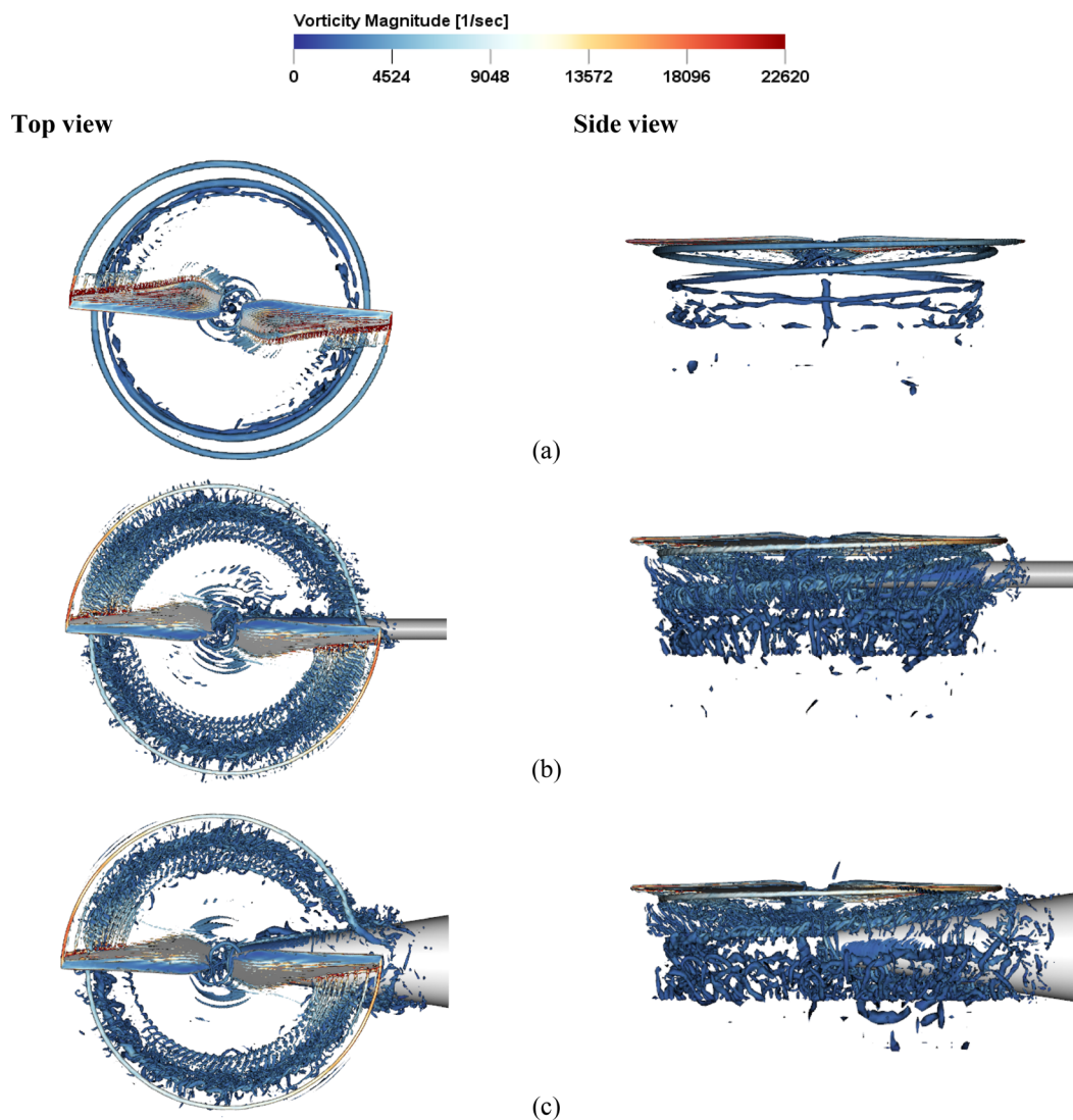
FIG. 16. Comparison of rotor wake visualized by iso-surfaces of the \Lambda_2 criterion: (a) isolated rotor, (b) rotor-cylinder airframe, and (c) rotor-conical airframe.
