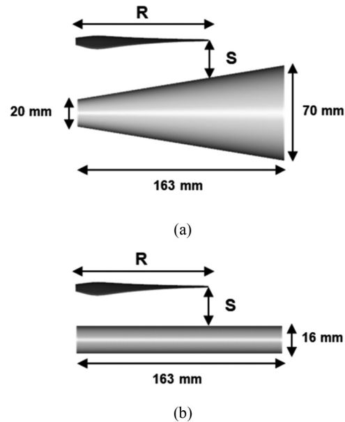
FIG. 4. Geometry of airframe: (a) conical airframe and (b) cylindrical airframe.
