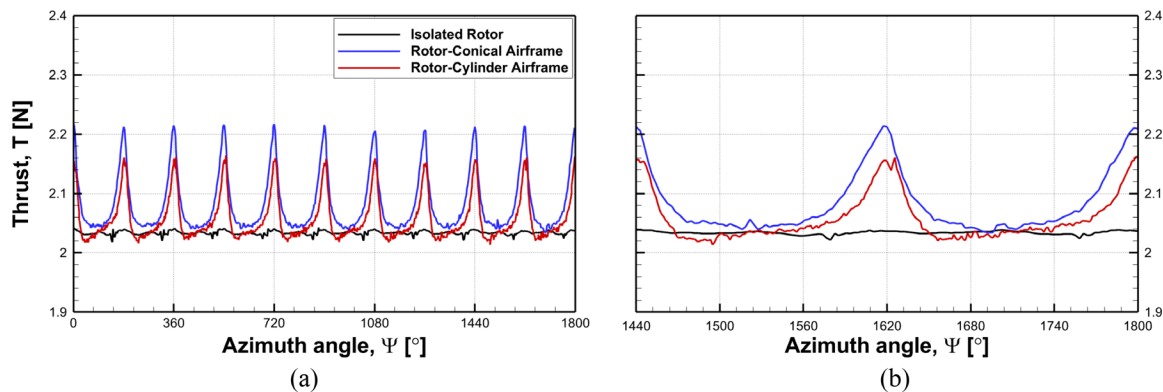
FIG. 12. Comparison of time-history of thrust forces between rotor–airframe and isolated rotor configurations: (a) 5 rev. and (b) 1 rev.
