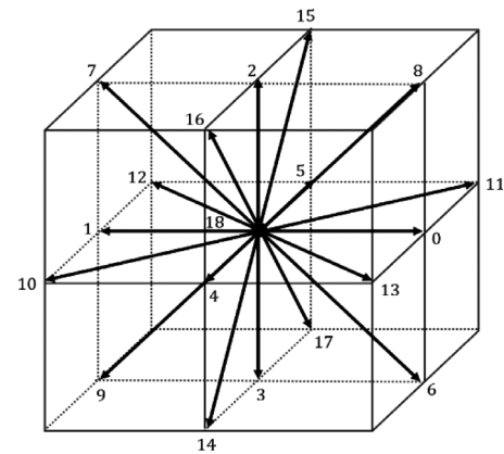
FIG. 1. D3Q19 model for discretizing the lattice-Boltzmann equation.
