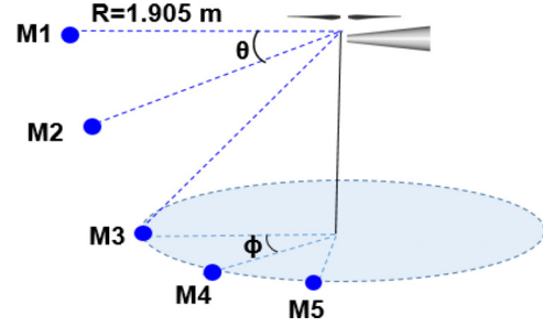
FIG. 7. Definition of microphone positions, azimuth angle ( \phi ), and elevation angle ( \theta ).
