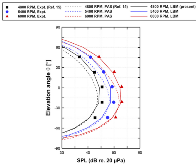
FIG. 9. Comparison of first BPF directivity between LBM simulations and measurements.
