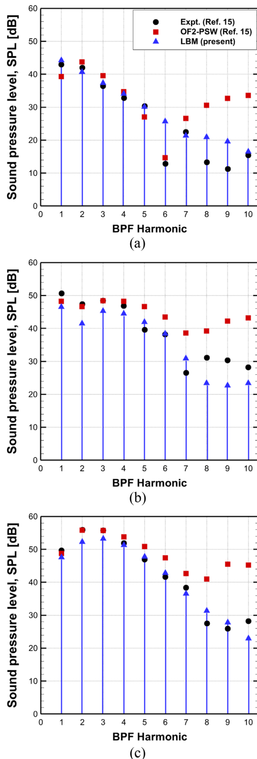
FIG. 11. Comparison of the amplitude of BPF harmonics between LBM simulations and measurements for conical airframe case: (a) M1, (b) M3, and (c) M5 locations.
