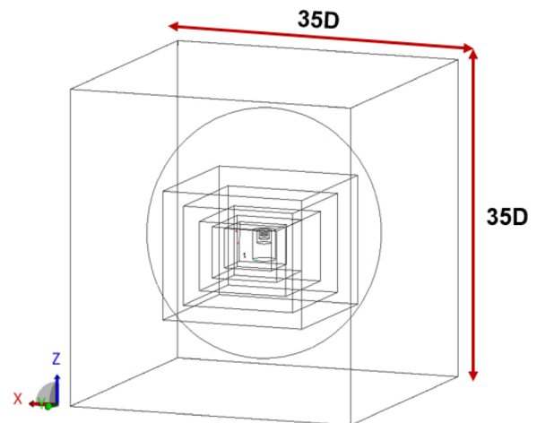
FIG. 5. Computational domain for LBM simulations.
