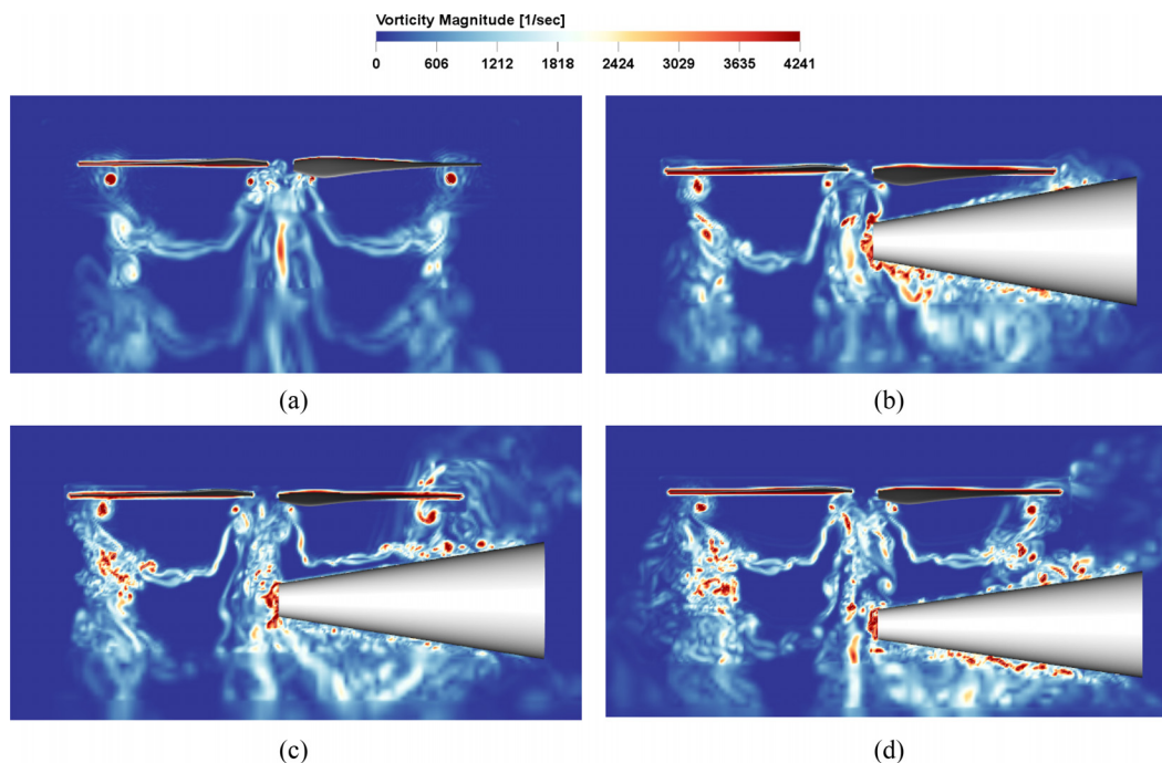
FIG. 18. Comparison of vorticity magnitude contours between isolated rotor and rotor-conical airframe configurations with different separation distances: (a) isolated rotor, (b) S/R = -0.1R , (c) S/R = -0.3 , and (d) S/R = -0.5 .
