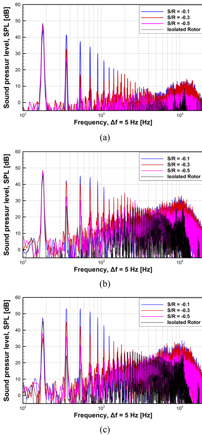
FIG. 19. Comparison of acoustic narrowband spectra between isolated rotor and rotor-conical airframe configurations with different separation distances: (a) M1, (b) M3, and (c) M5 locations.
