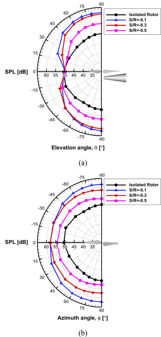
FIG. 20. Comparison of overall sound pressure level (OASPL) directivity between the isolated rotor and rotor-conical airframe with different separation distances: (a) elevation angle and (b) azimuth angle.
