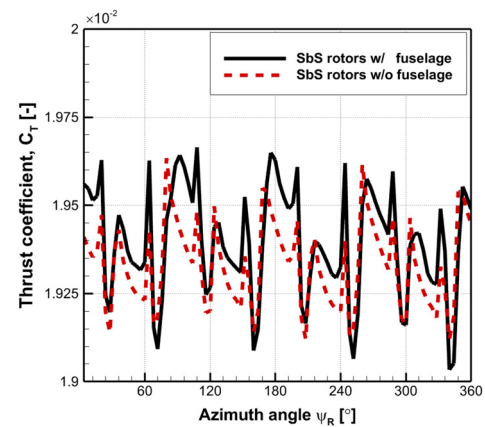
FIG. 11. Time variation in thrust coefficient for one revolution of isolated rotor and full configuration.
