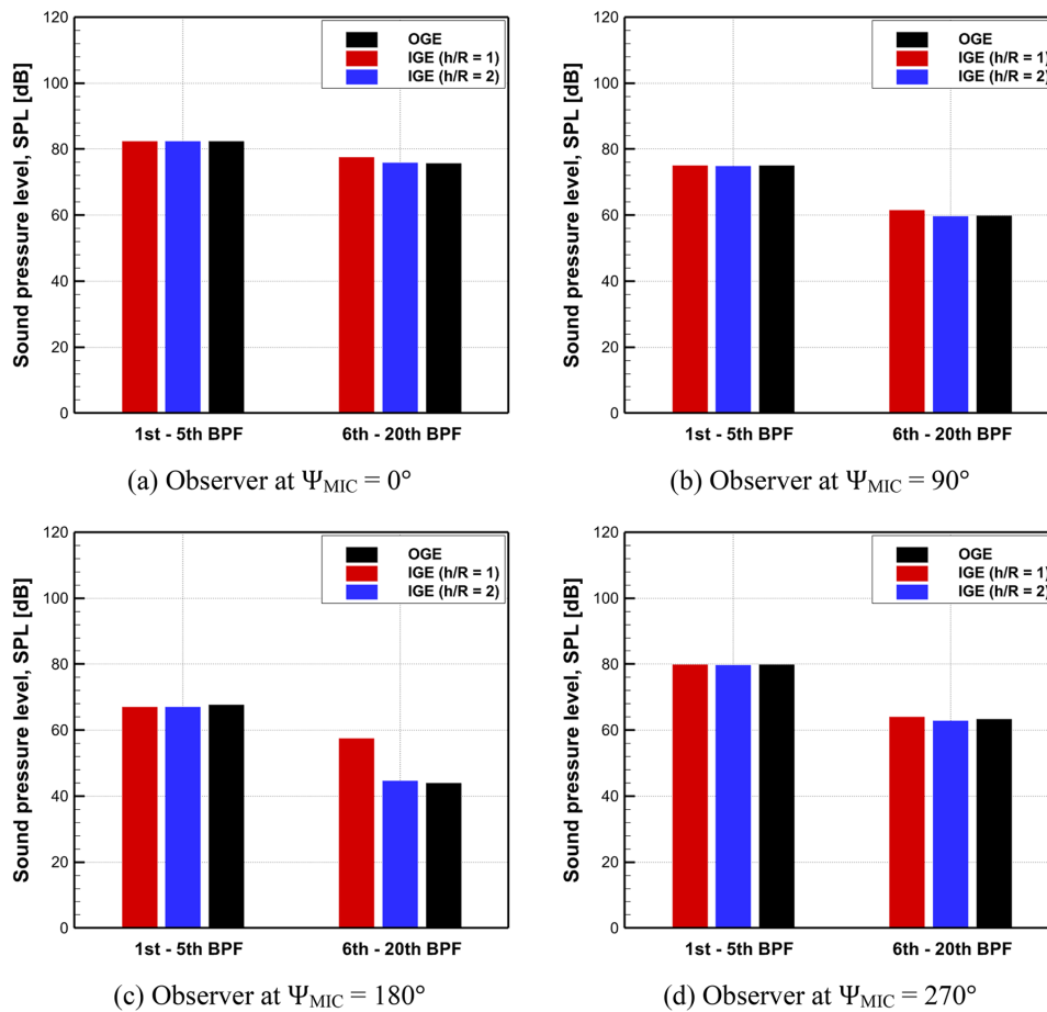
FIG. 22. Accumulated sound pressure levels calculated from 1–5 BPF and 6–20 BPF.
