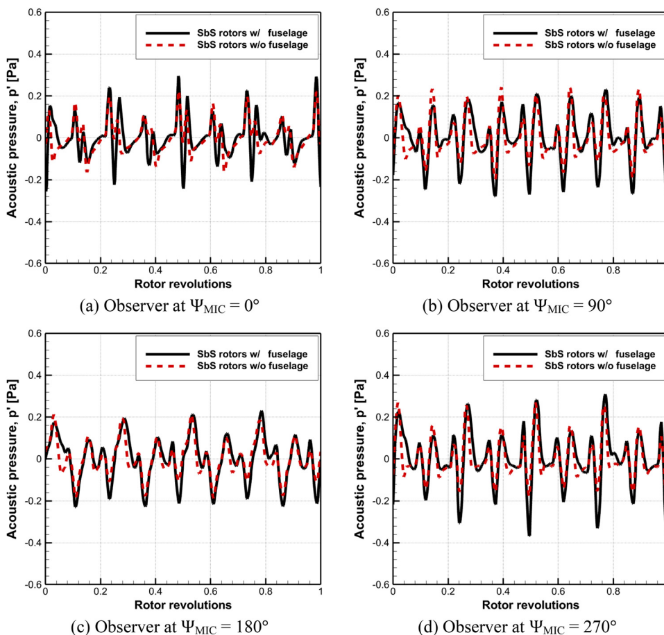
FIG. 12. Comparison of the overall acoustic pressure for isolated rotor and full configuration in hovering condition with OGE.
