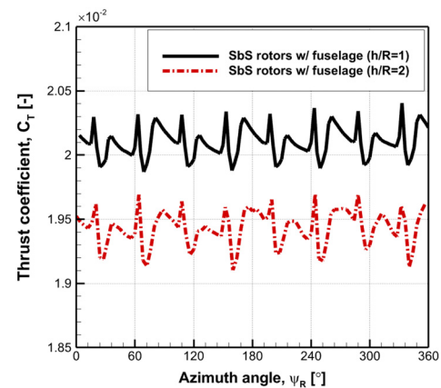
FIG. 15. Time variation in thrust coefficient for one rotor revolution of full configuration in IGE conditions.
