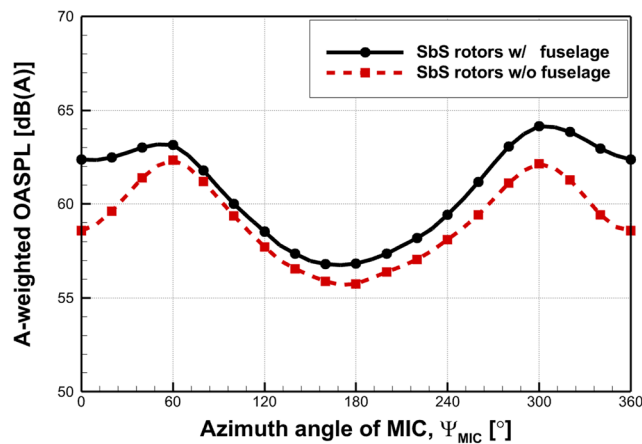
FIG. 14. Comparison of A-weighted overall sound pressure levels (OASPLs) for isolated rotor and full configuration aircraft at various observer positions.
