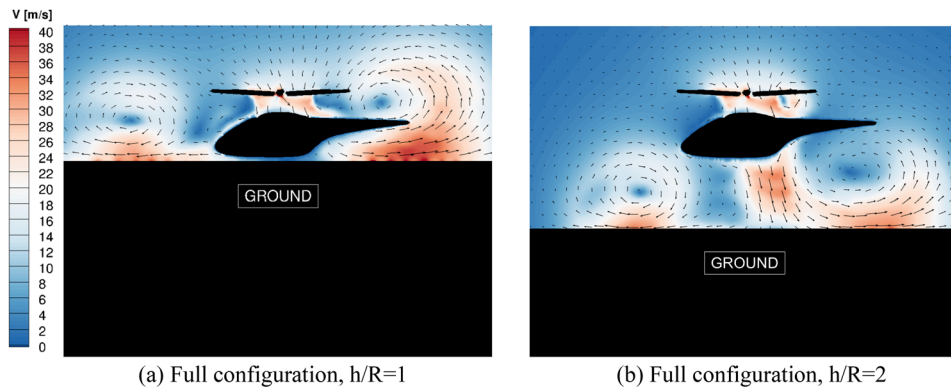
FIG. 17. Comparison of the instantaneous velocity magnitude contour of full configuration in IGE conditions.
