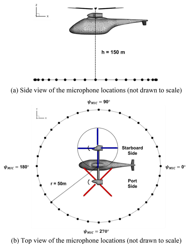
FIG. 7. Acoustics simulation setup: microphone locations.
