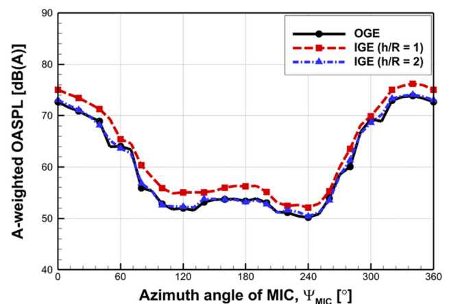
FIG. 23. A-weighted overall sound pressure levels (OASPLs) of UAM aircraft in ground effect (IGE) at various observer positions.
