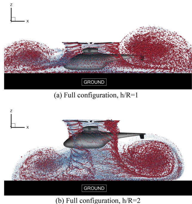
FIG. 18. Comparison of wake structures of full configuration in IGE conditions.
