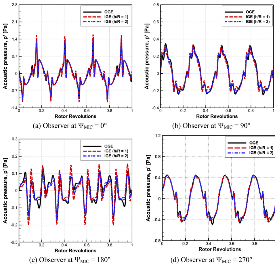
FIG. 20. Comparison of the overall acoustic pressure for hovering UAM aircraft in ground effect (IGE) at h/R = 1 and 2 .
