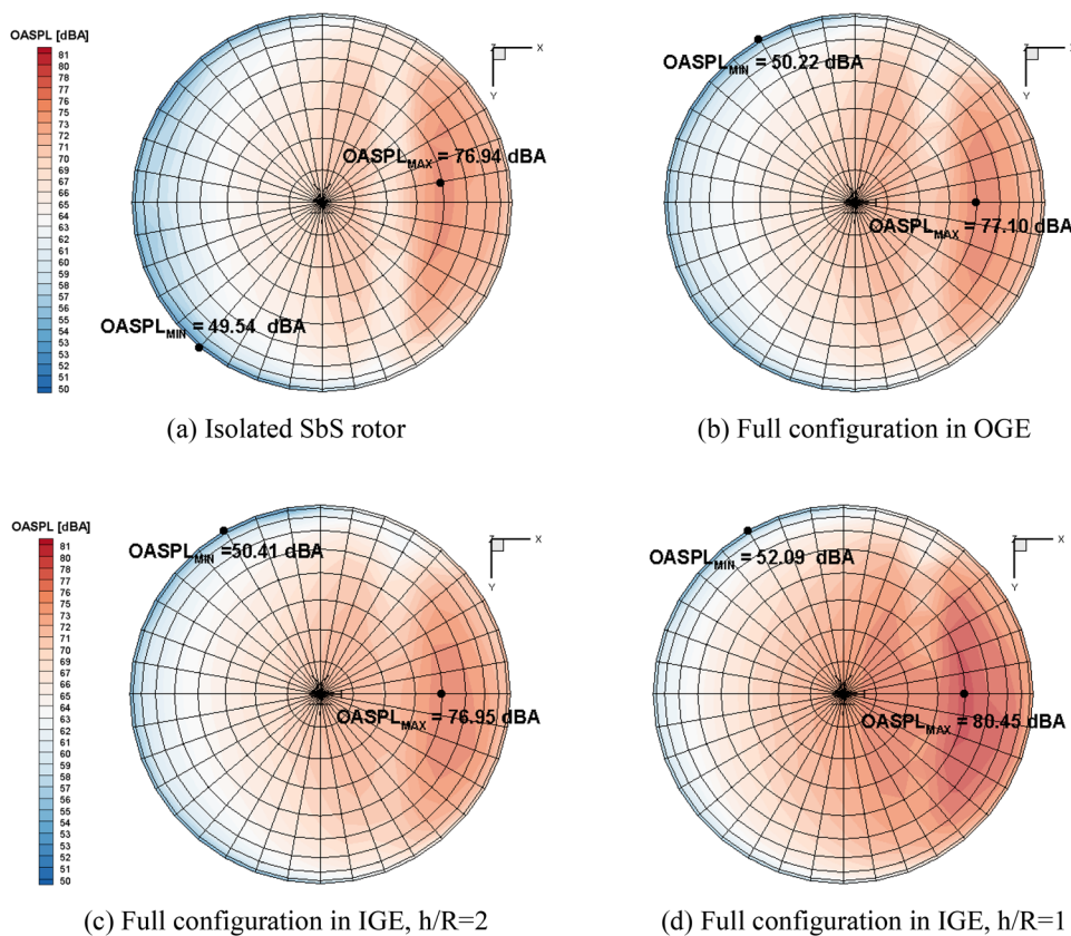
FIG. 24. Three-dimensional representation of OASPL evaluated on the hemisphere above the rotor system with the radius of 50 m from the center of the rotors (bottom-side view).
