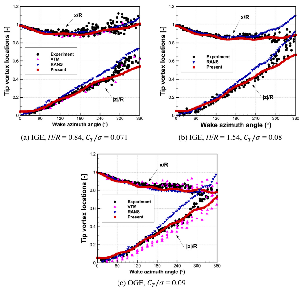
FIG. 5. Tip vortex axial and radial locations of the Lynx tail rotor.
