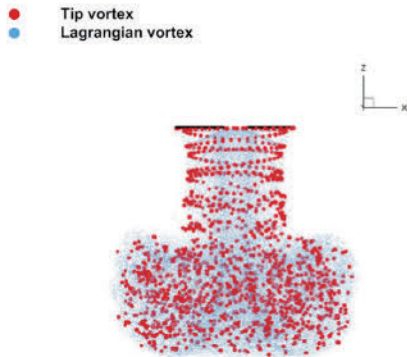
Fig. 3. Wake structure of Caradonna-Tung rotor blade at collective pitch angle of 8^\circ
