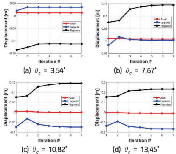
Fig. 15. Tip displacement at each iteration
