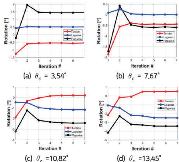
Fig. 16. Tip rotation at each iteration
