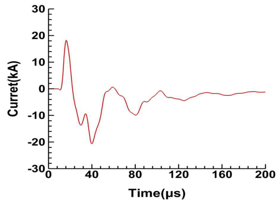
Fig. 17 Current monitor result at the nose depending on the time domain
