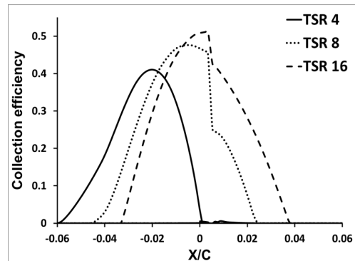
Fig. 5. Collection efficiency at various tip speed ratios
