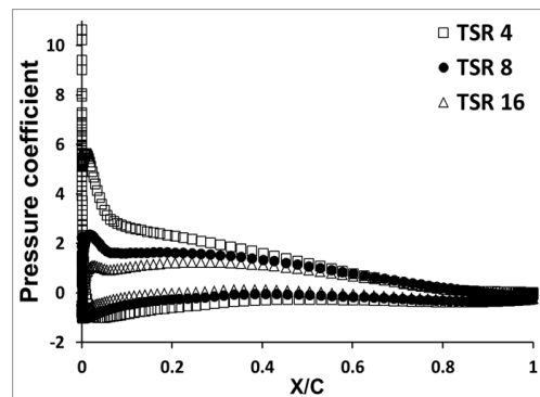
Fig. 3. Pressure coefficients at various tip speed ratios
