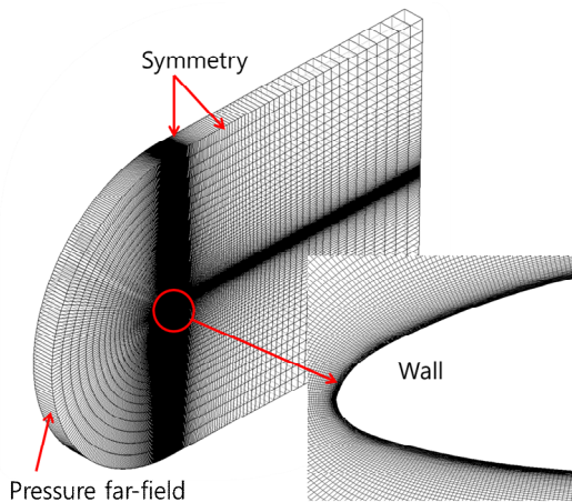
Fig. 2. Global view of mesh
