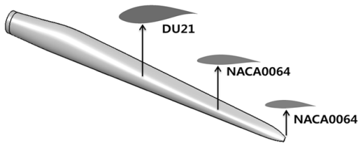
Fig. 1. 3D CAD of NREL 5MW wind turbine blade
