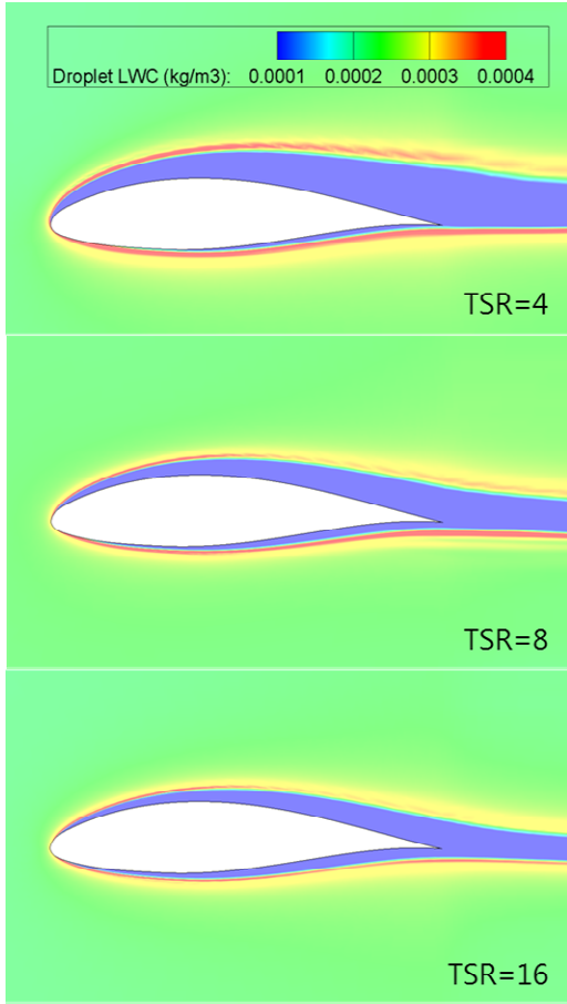
Fig. 4. LWC distributions at various tip speed ratios
