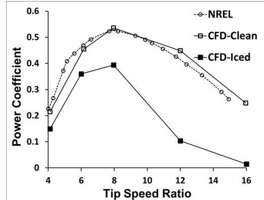
Fig. 10. Comparison of power coefficient versus tip speed ratio (clean and iced)
