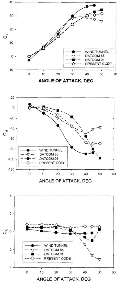
Fig. 3. Force and moment coefficients for 0-degree roll and deflection angle
