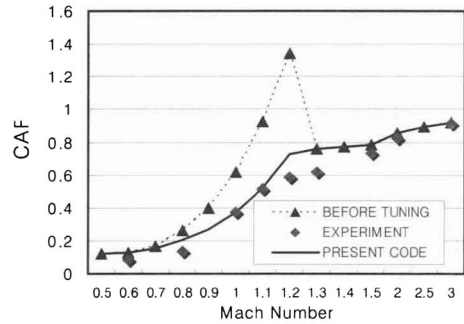
Fig. 6. Comparison of forebody axial force coefficient in transonic flow around a hemispherical nose
